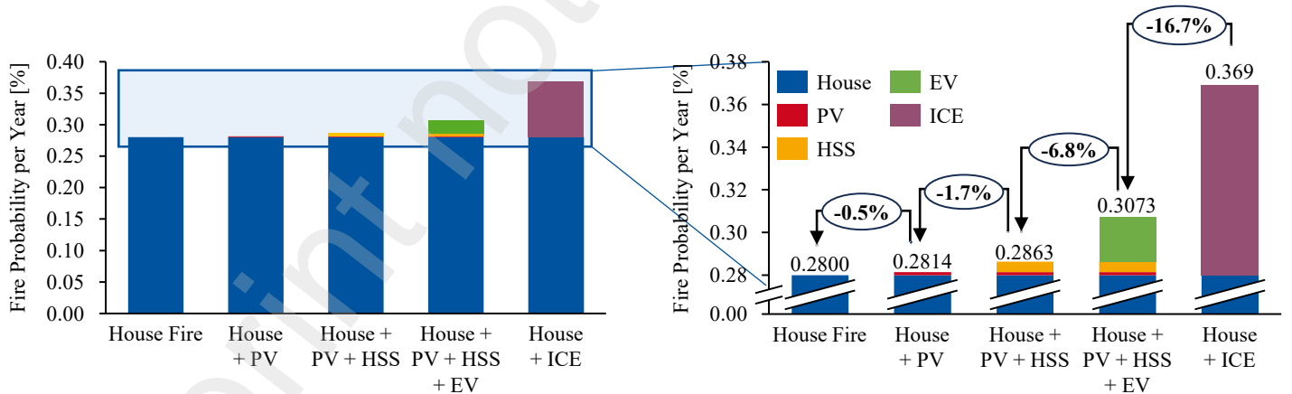
Figure 13: Posed annual fire risk for the considered case study possessing the combination of different systems.
