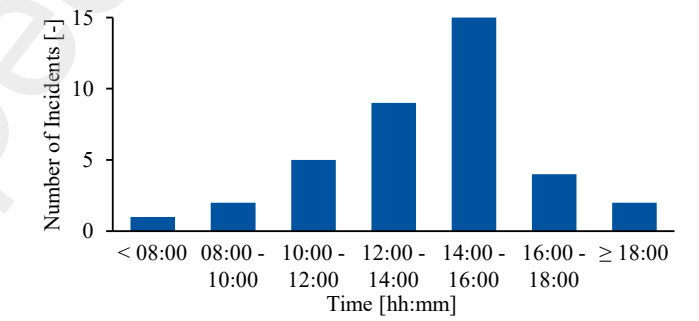
Figure 10: Distribution of the fire incidents analyzed in 2022 and 2023 over the time of day.
