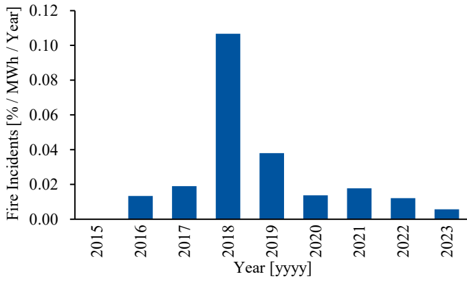
Figure 7: Fire risk of large-scale BESS. Illustration based on [23–25].
