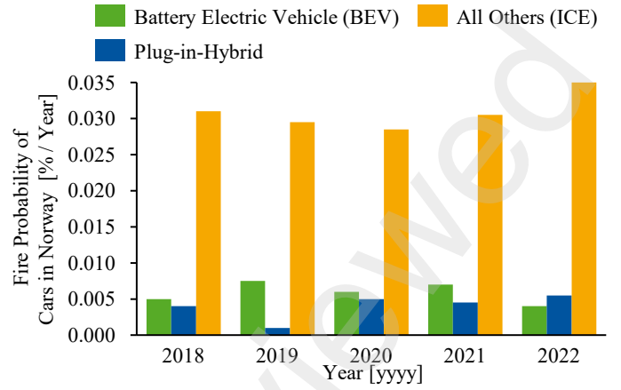
Figure 6: Fire probability of vehicle categories per year in Norway. Illustration based on [22].
