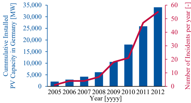
Figure 3: Increasing number of PV-triggered fires with increasing installed capacity in Germany. Illustration based on [18,31].
