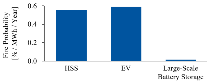
Figure 11: Comparison of fire probabilities per MWh.
